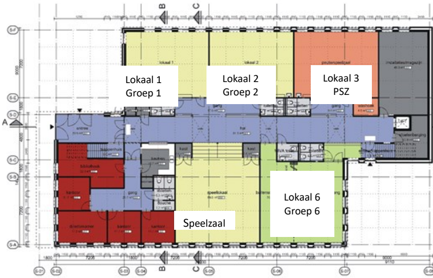
begane grond 1:200
